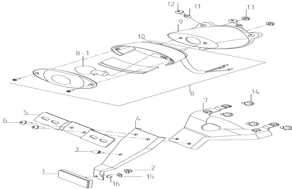
FIG.15 TAIL LIGHT
