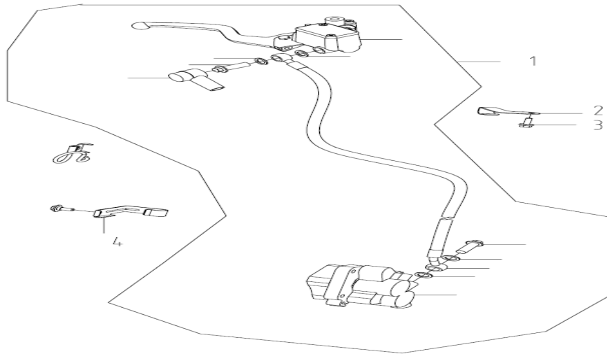
FIG.23 FRONT BRAKE
