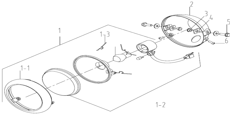
FIG.17 HEADLIGHT
