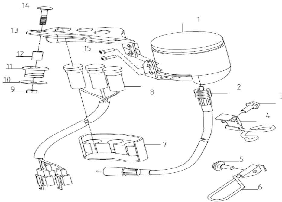
FIG.3 SPEEDOMETER
