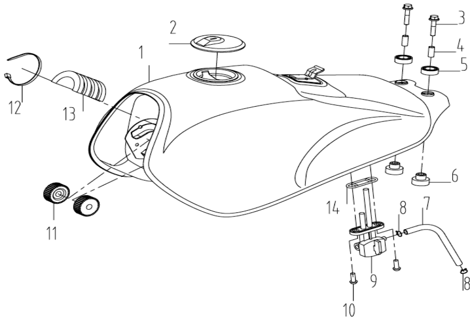
FIG.2 FUEL TANK
