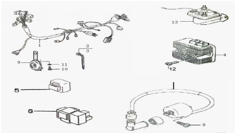
FIG.25 WIRING HARNESS
