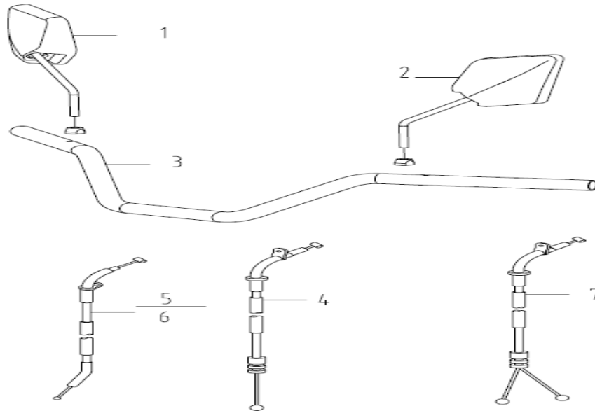
FIG.20 REAR MIRROR
